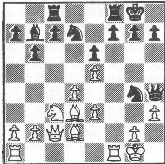
140 After 15 h3
